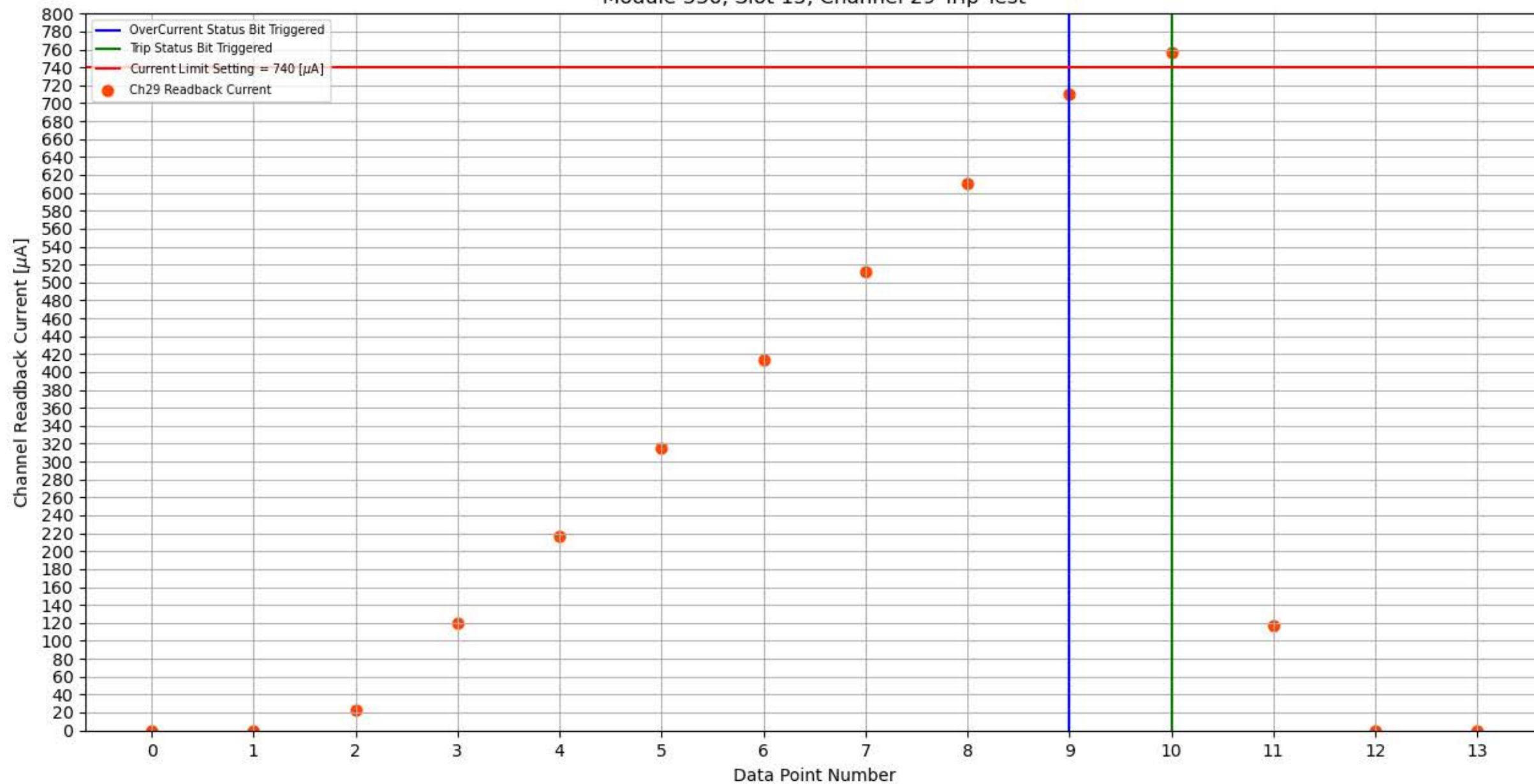
Module 336, Slot 15, Channel 29 Trip Test
