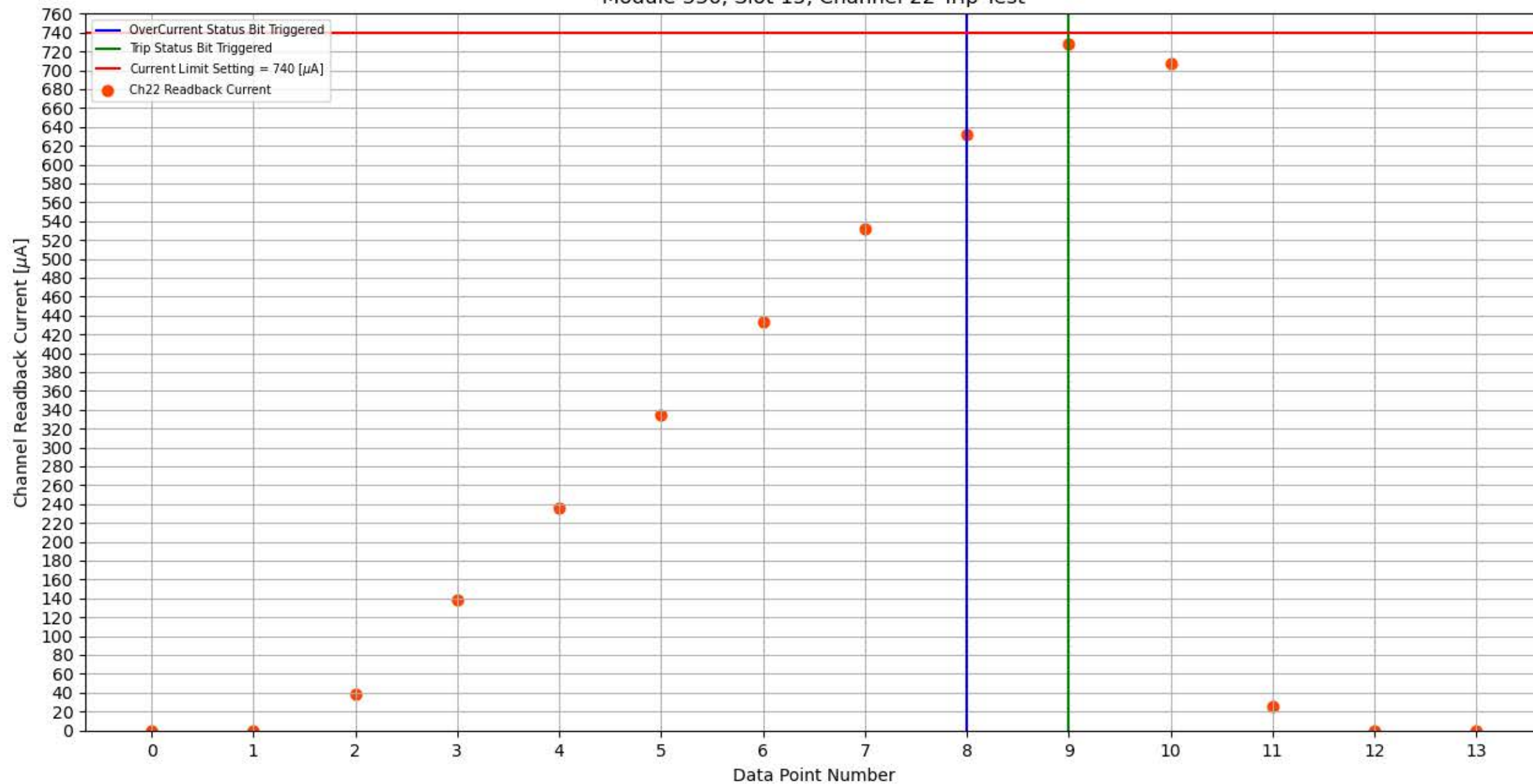
Module 336, Slot 15, Channel 22 Trip Test
