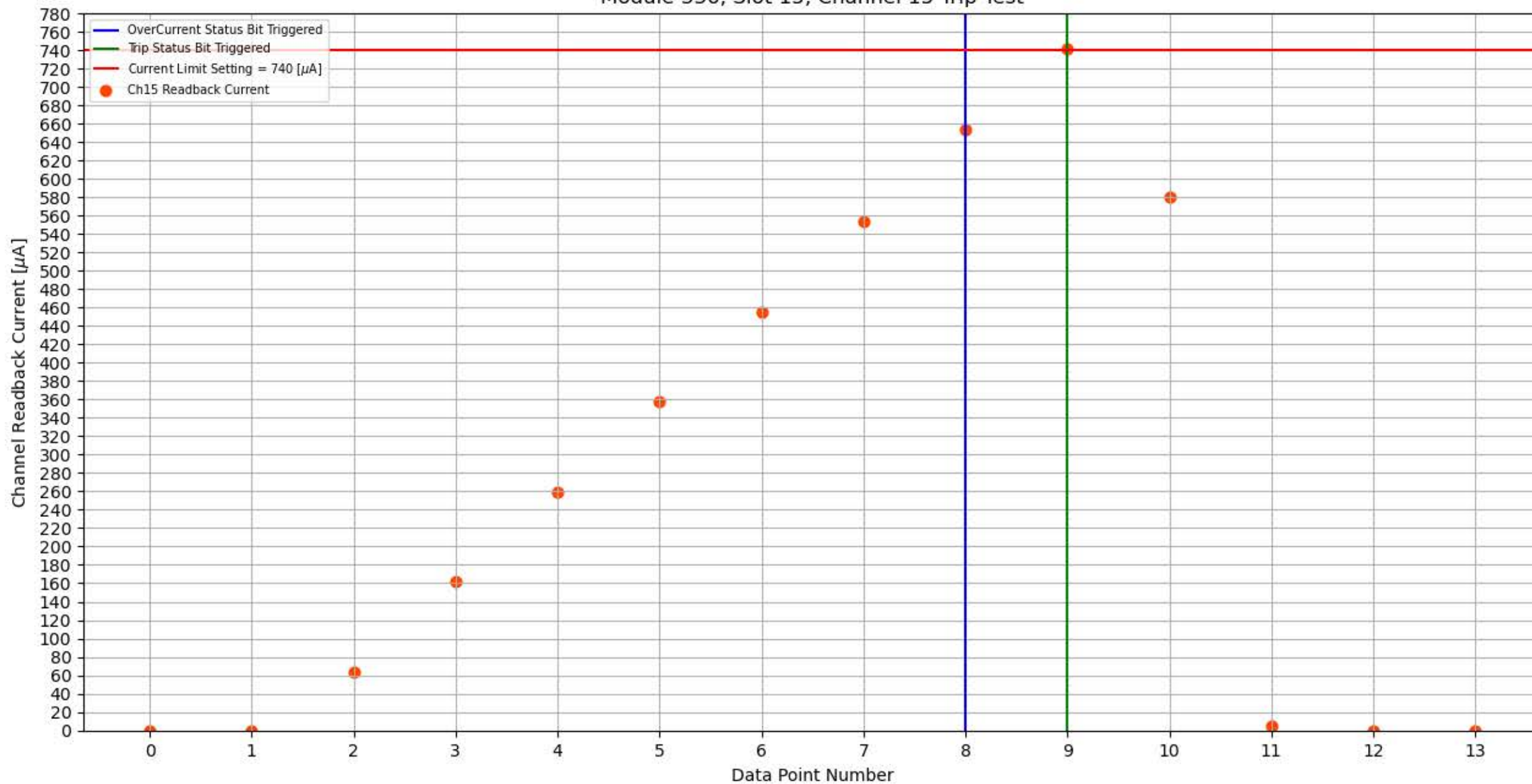
Module 336, Slot 15, Channel 15 Trip Test
