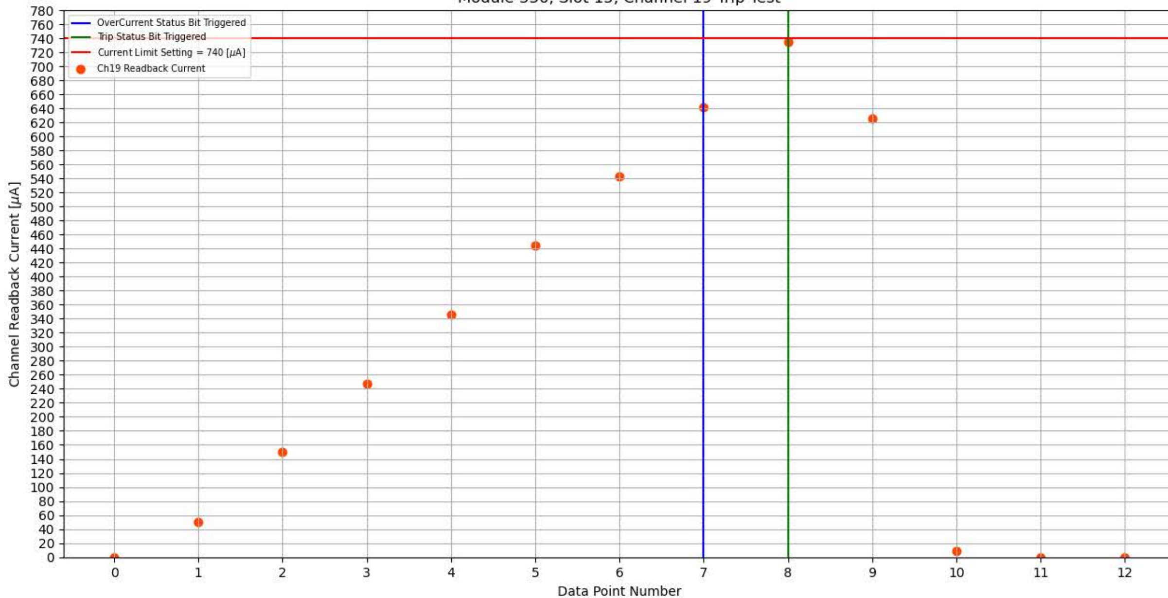
Module 336, Slot 15, Channel 19 Trip Test
