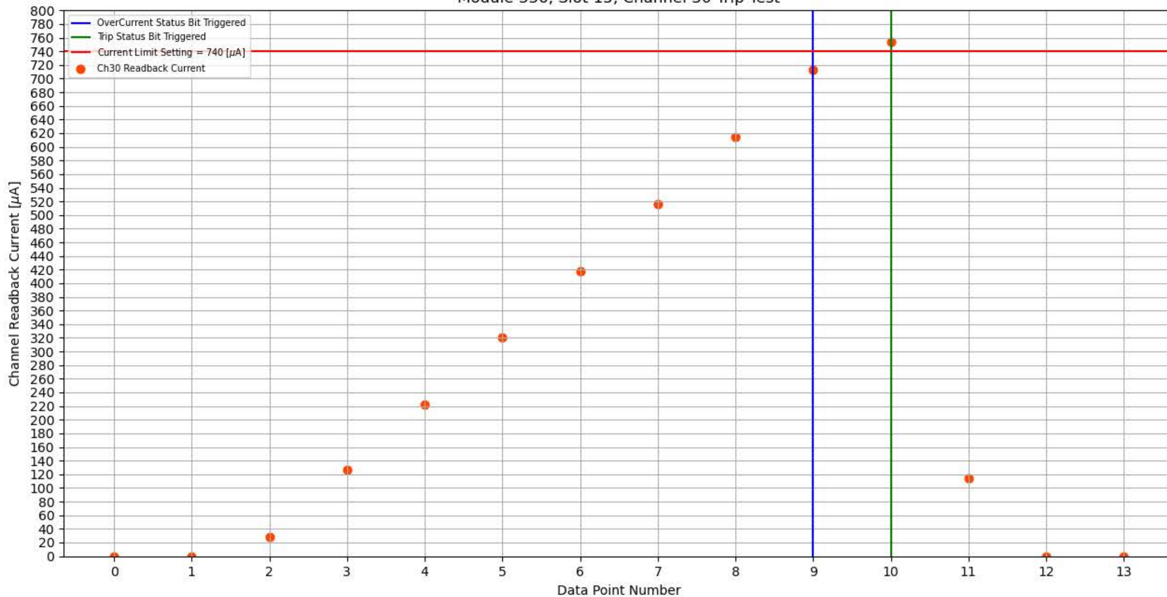
Module 336, Slot 15, Channel 30 Trip Test
