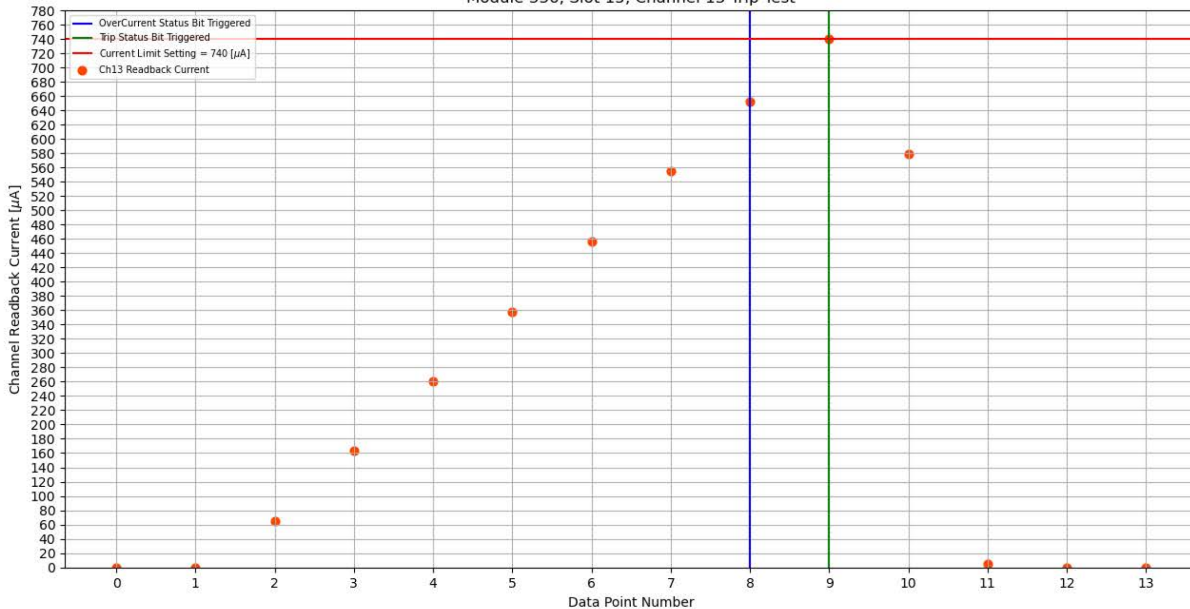
Module 336, Slot 15, Channel 13 Trip Test
