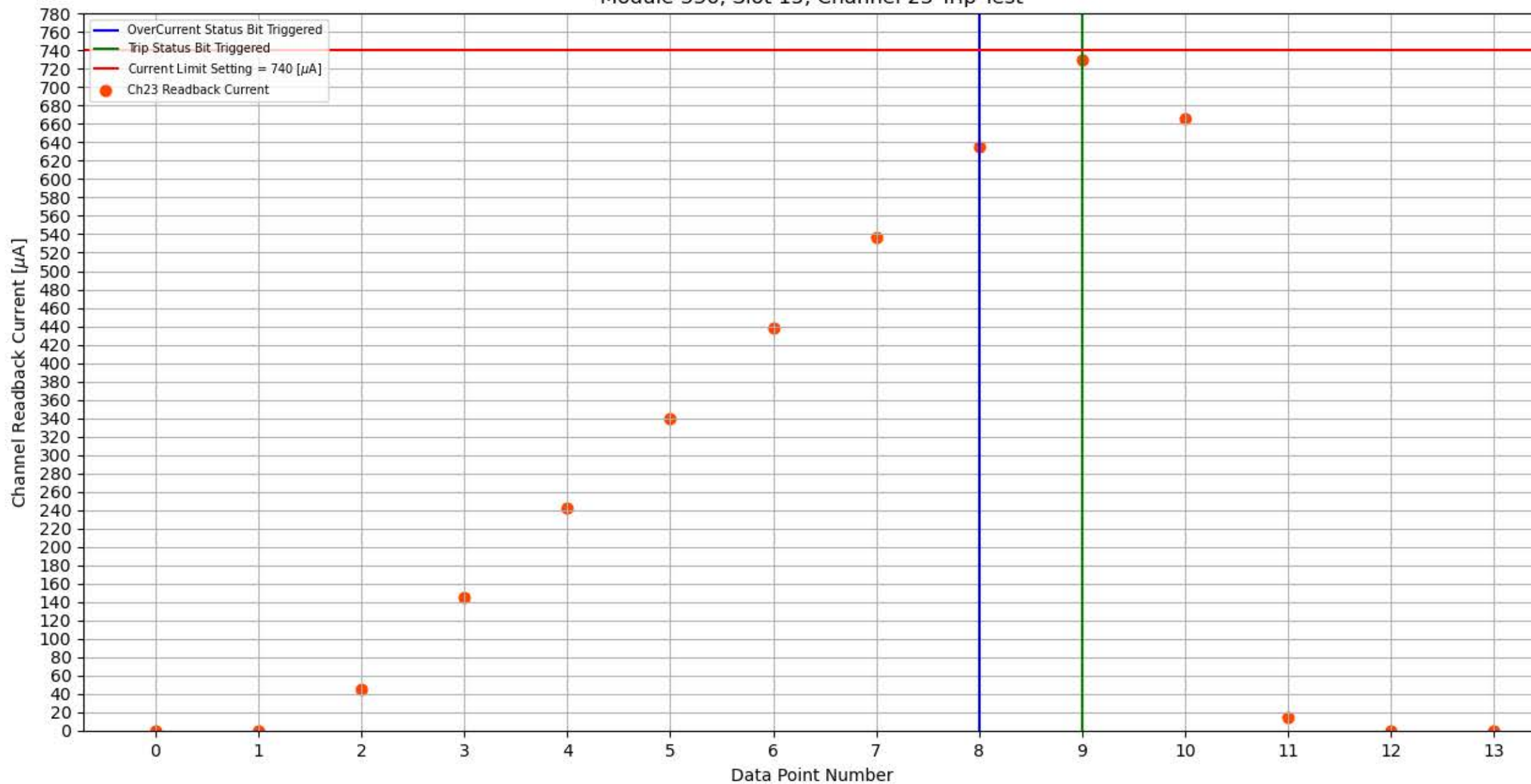
Module 336, Slot 15, Channel 23 Trip Test
