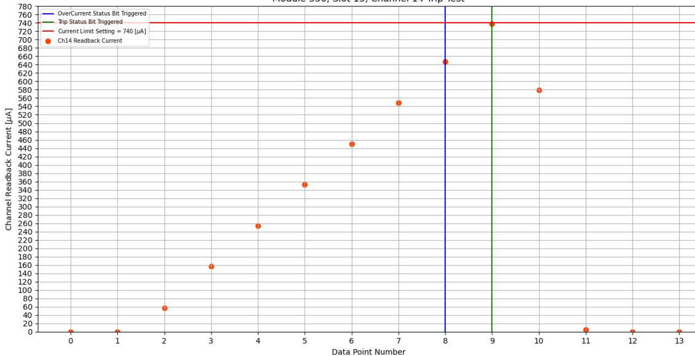
Module 336, Slot 15, Channel 14 Trip Test
