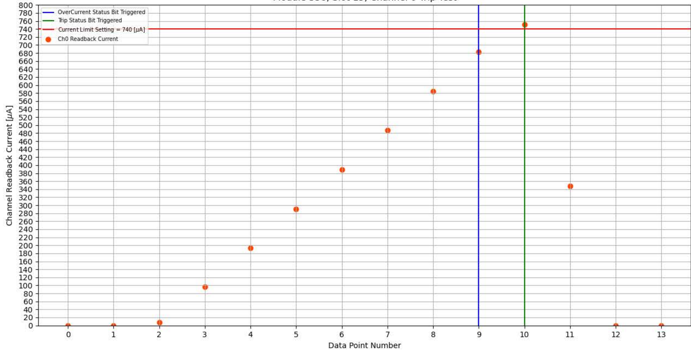
Module 336, Slot 15, Channel 0 Trip Test
