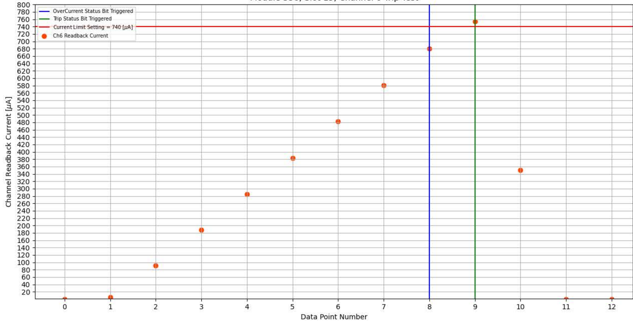
Module 336, Slot 15, Channel 6 Trip Test
