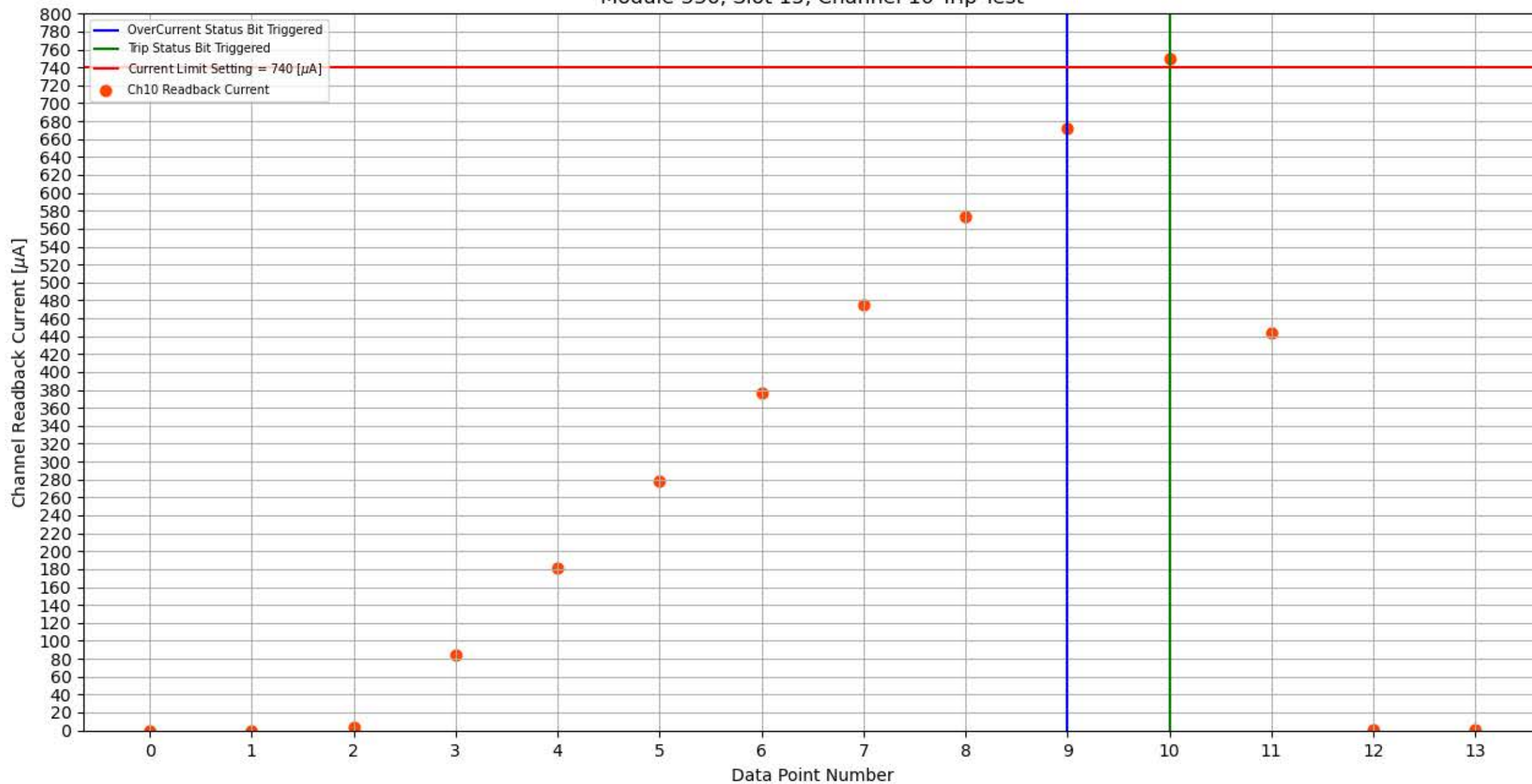
Module 336, Slot 15, Channel 10 Trip Test
