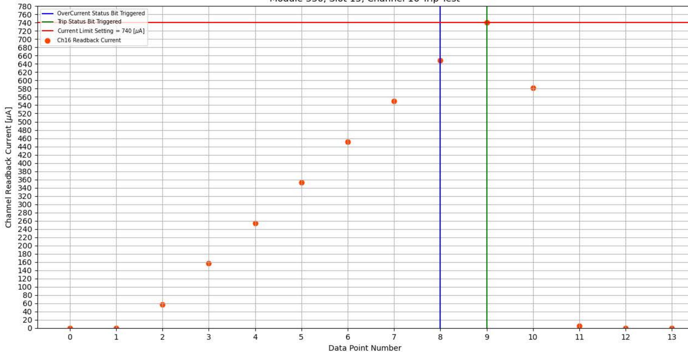
Module 336, Slot 15, Channel 16 Trip Test
