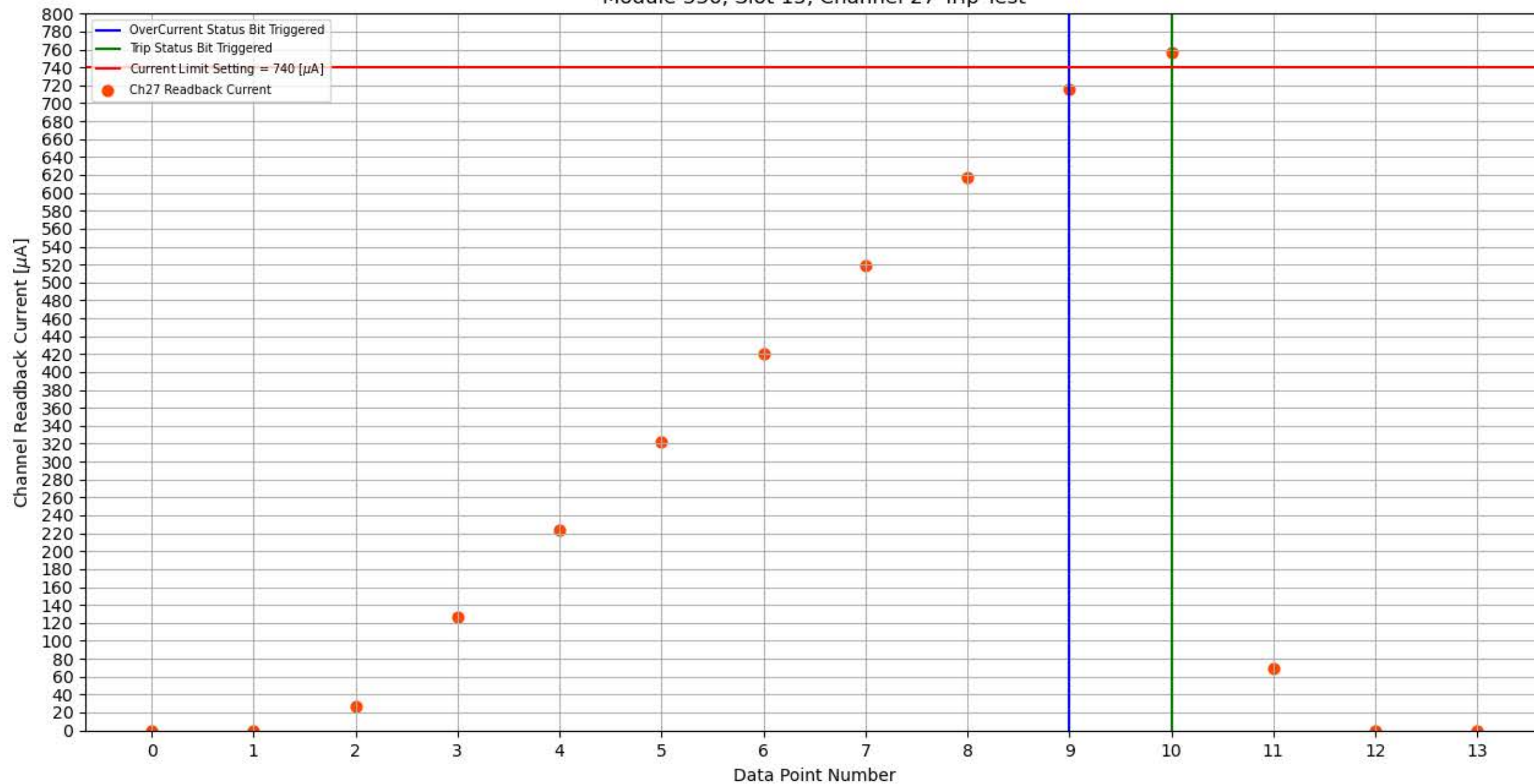
Module 336, Slot 15, Channel 27 Trip Test
