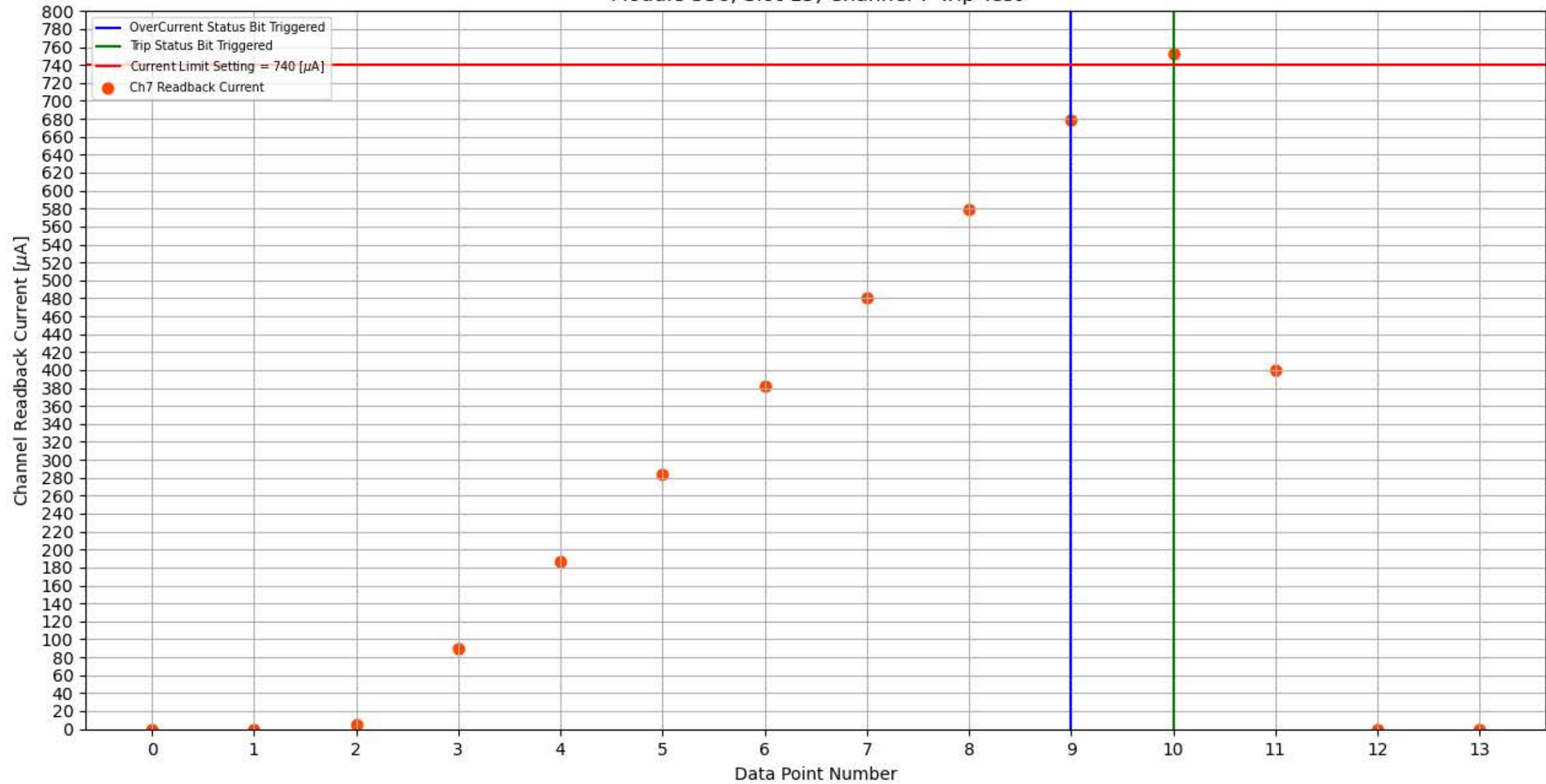
Module 336, Slot 15, Channel 7 Trip Test
