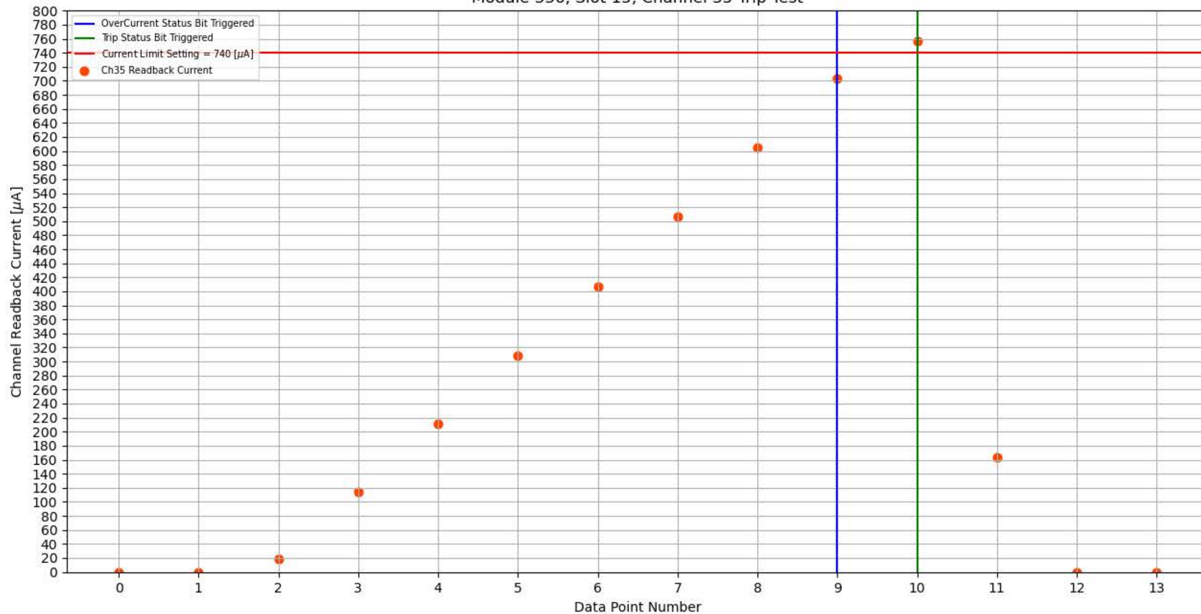
Module 336, Slot 15, Channel 35 Trip Test
