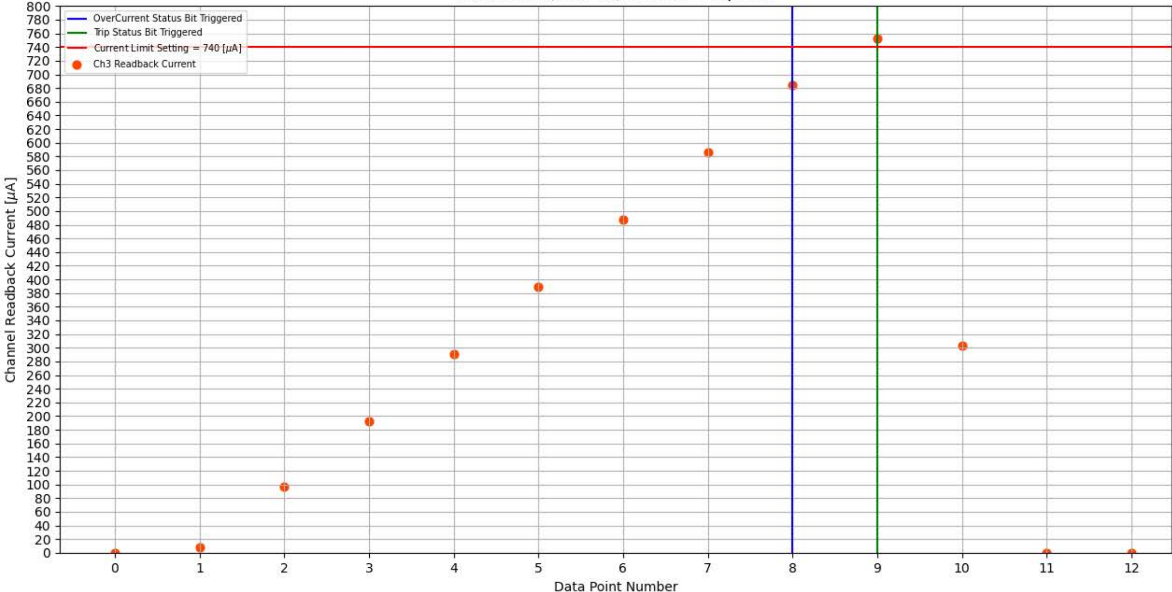
Module 336, Slot 15, Channel 3 Trip Test
