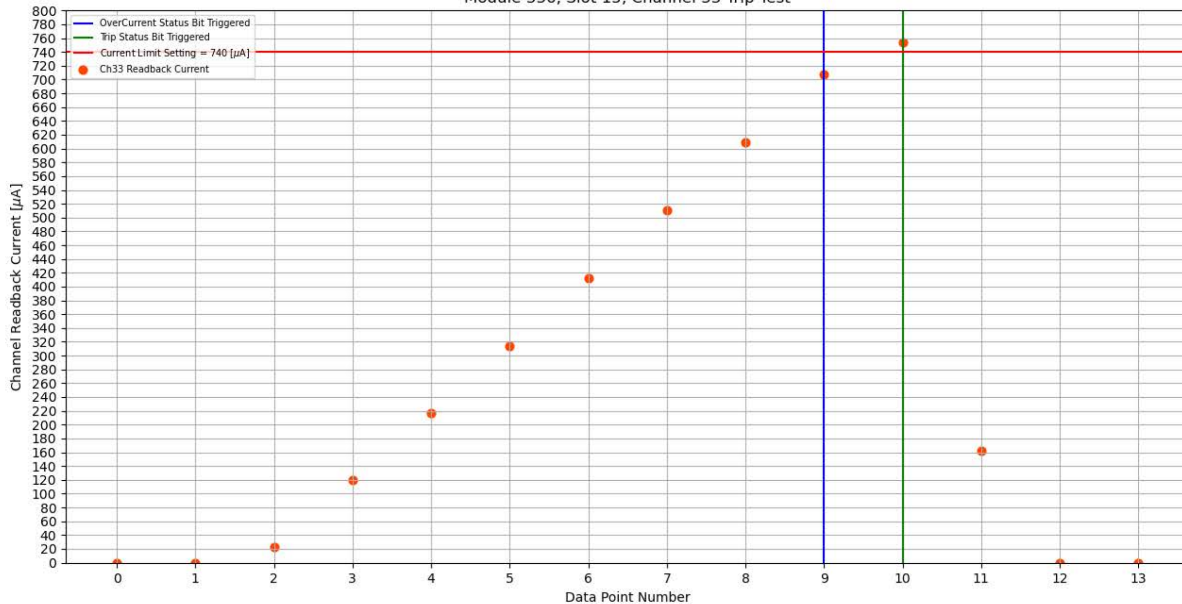
Module 336, Slot 15, Channel 33 Trip Test
