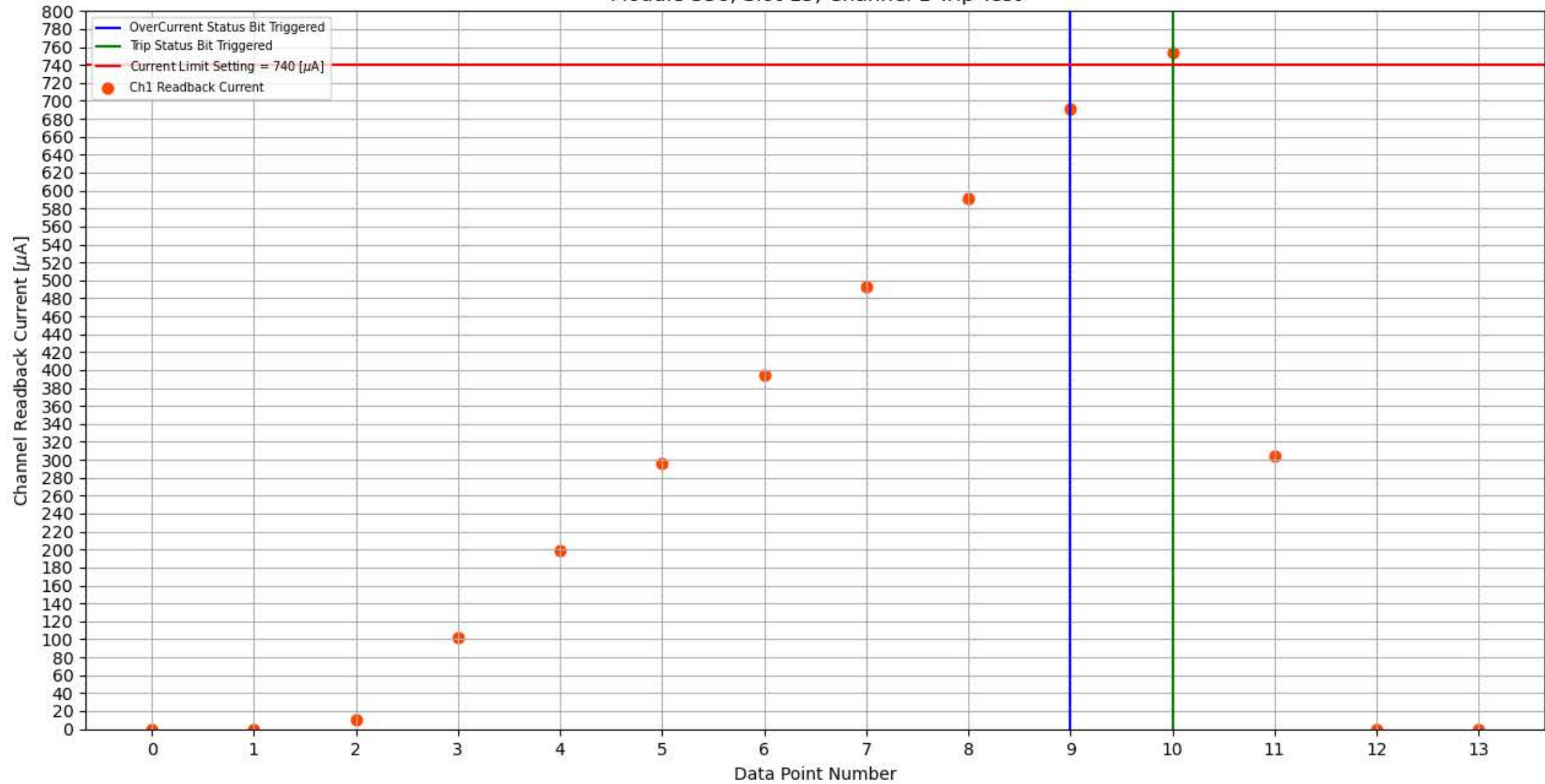
Module 336, Slot 15, Channel 1 Trip Test
