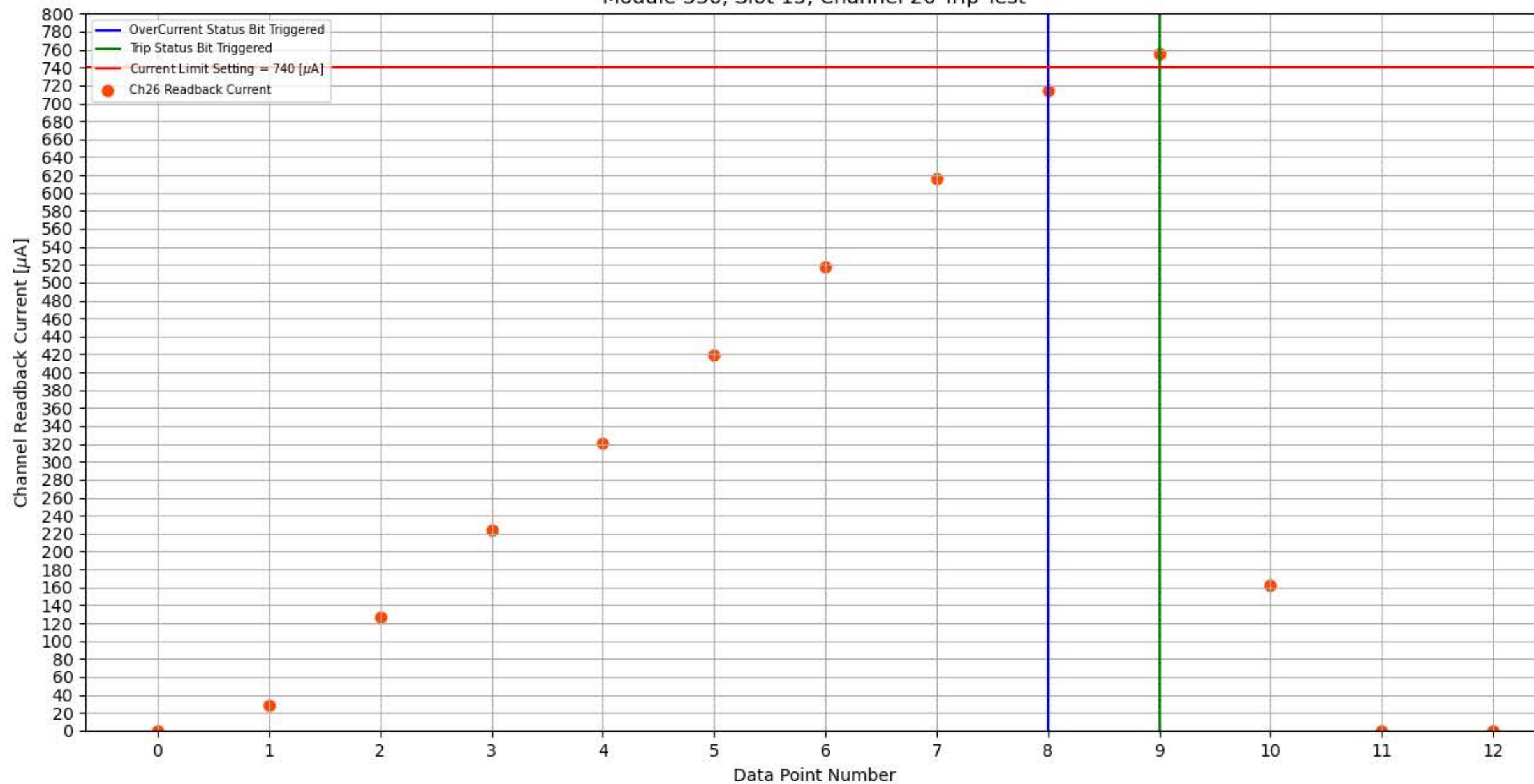
Module 336, Slot 15, Channel 26 Trip Test
