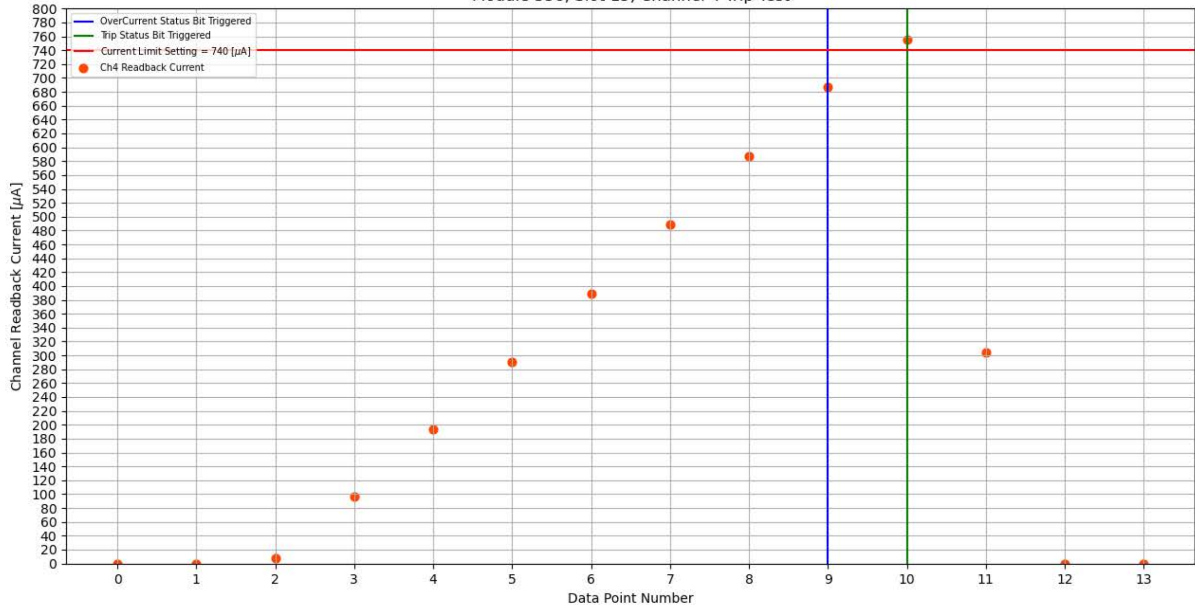
Module 336, Slot 15, Channel 4 Trip Test
