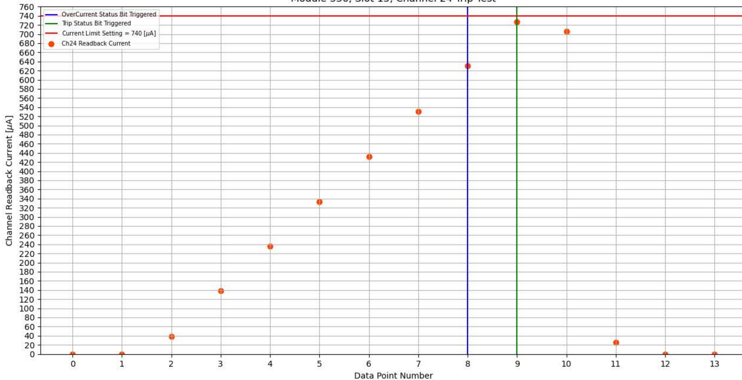
Module 336, Slot 15, Channel 24 Trip Test
