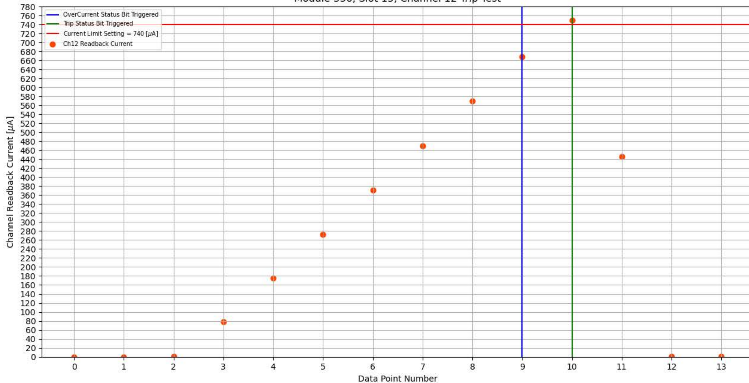
Module 336, Slot 15, Channel 12 Trip Test
