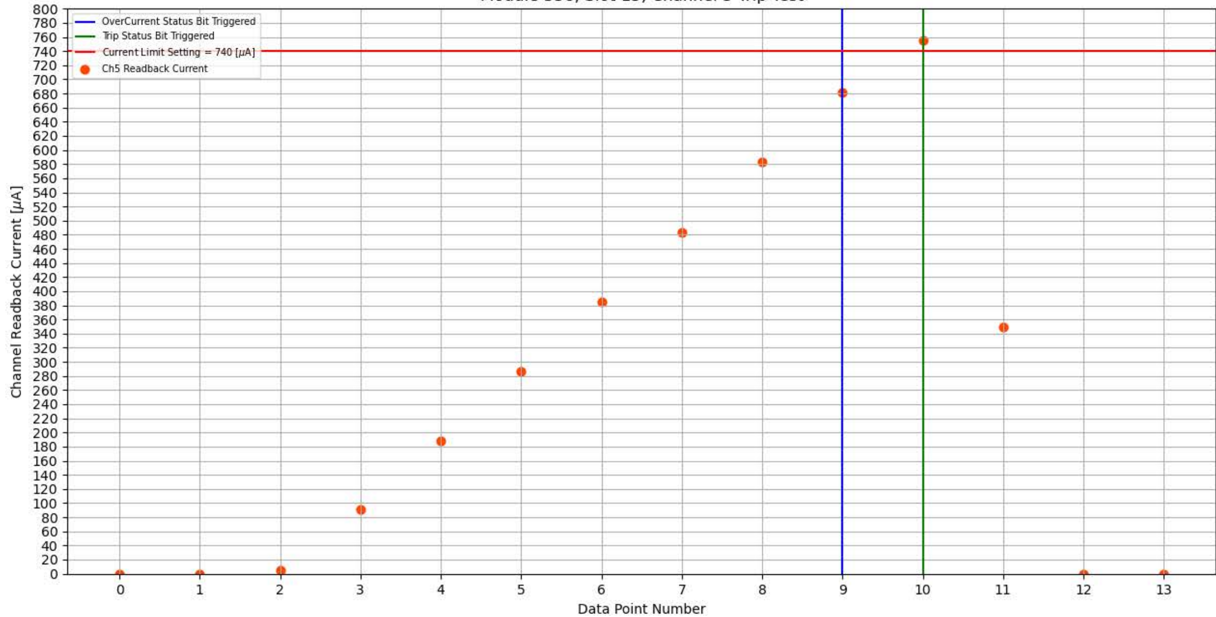
Module 336, Slot 15, Channel 5 Trip Test
