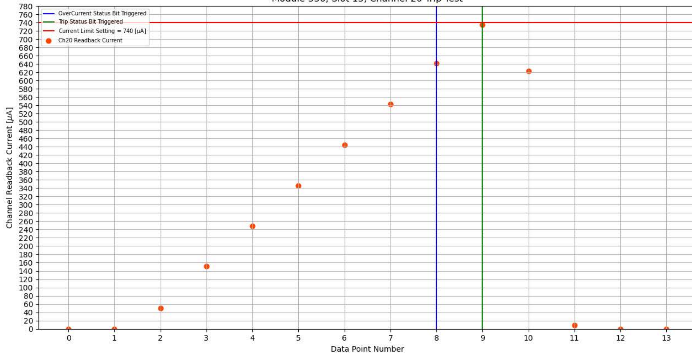
Module 336, Slot 15, Channel 20 Trip Test
