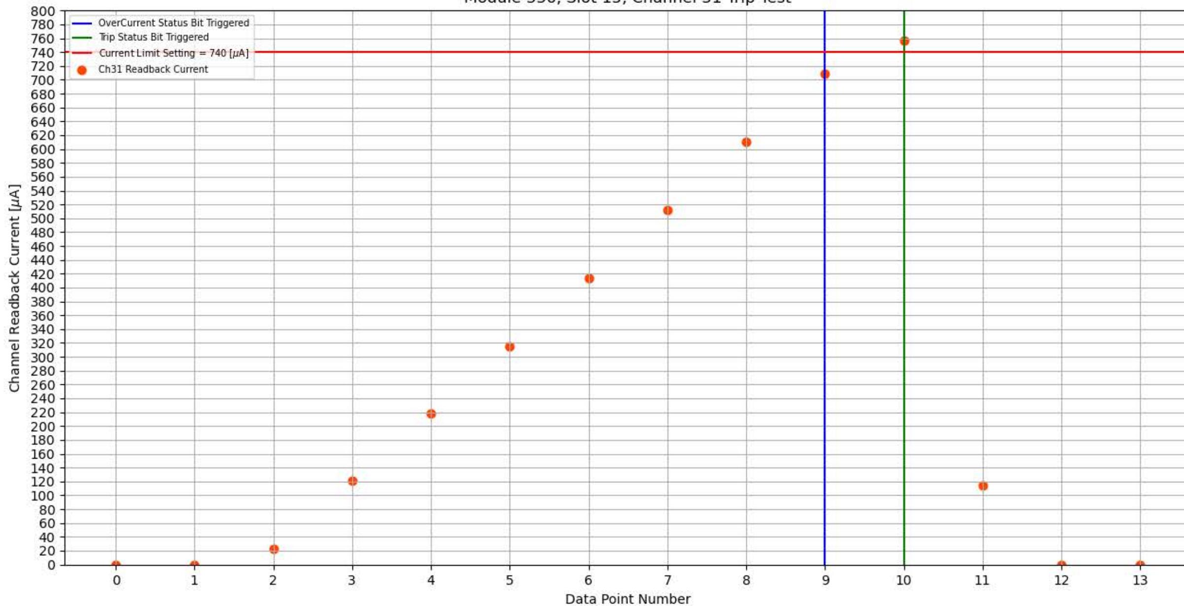
Module 336, Slot 15, Channel 31 Trip Test
