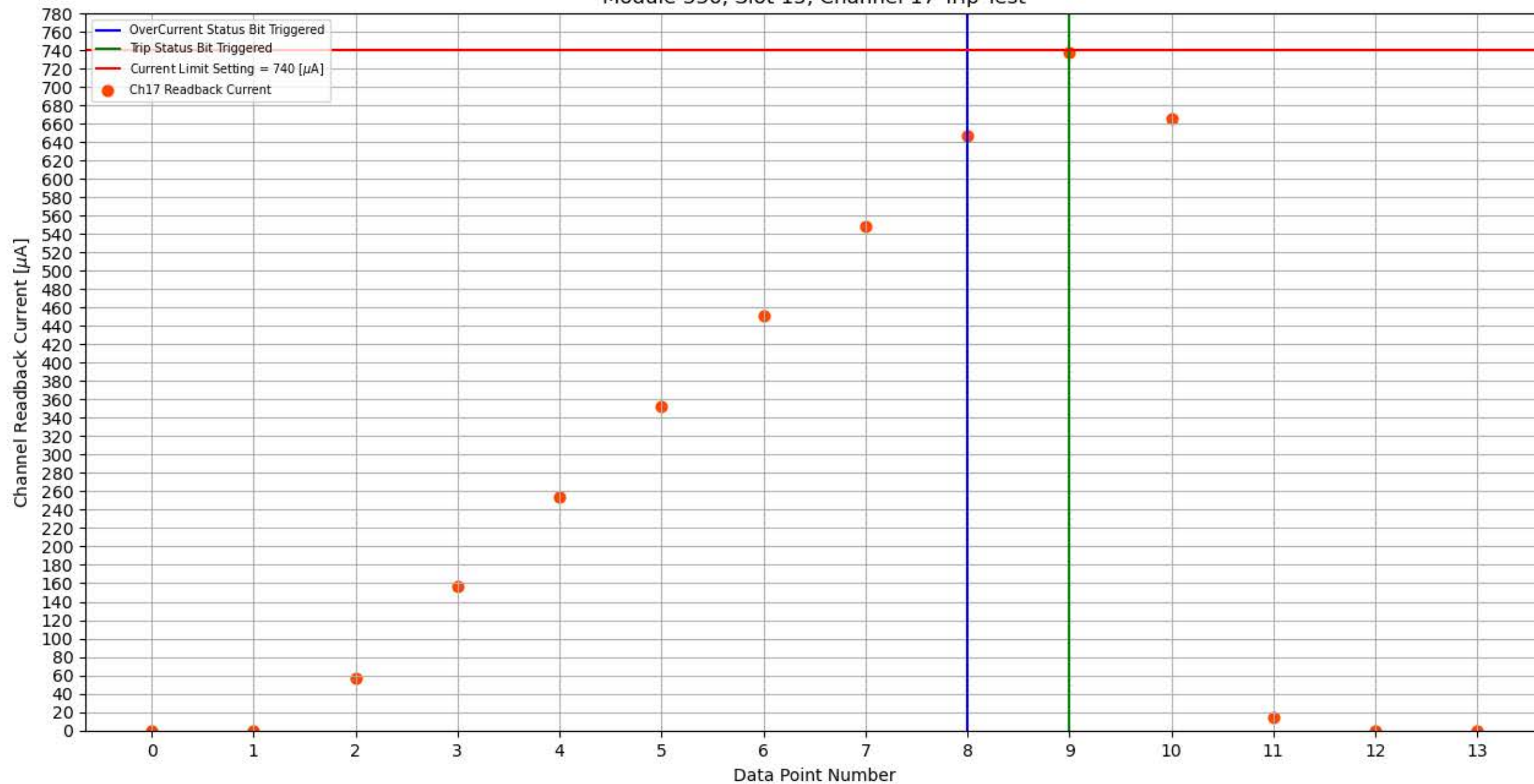
Module 336, Slot 15, Channel 17 Trip Test
