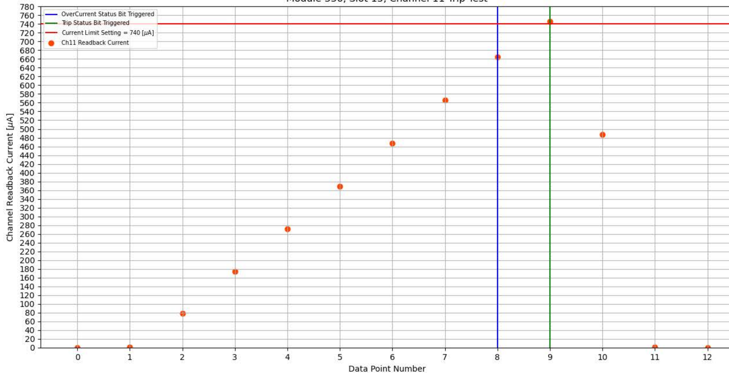
Module 336, Slot 15, Channel 11 Trip Test
