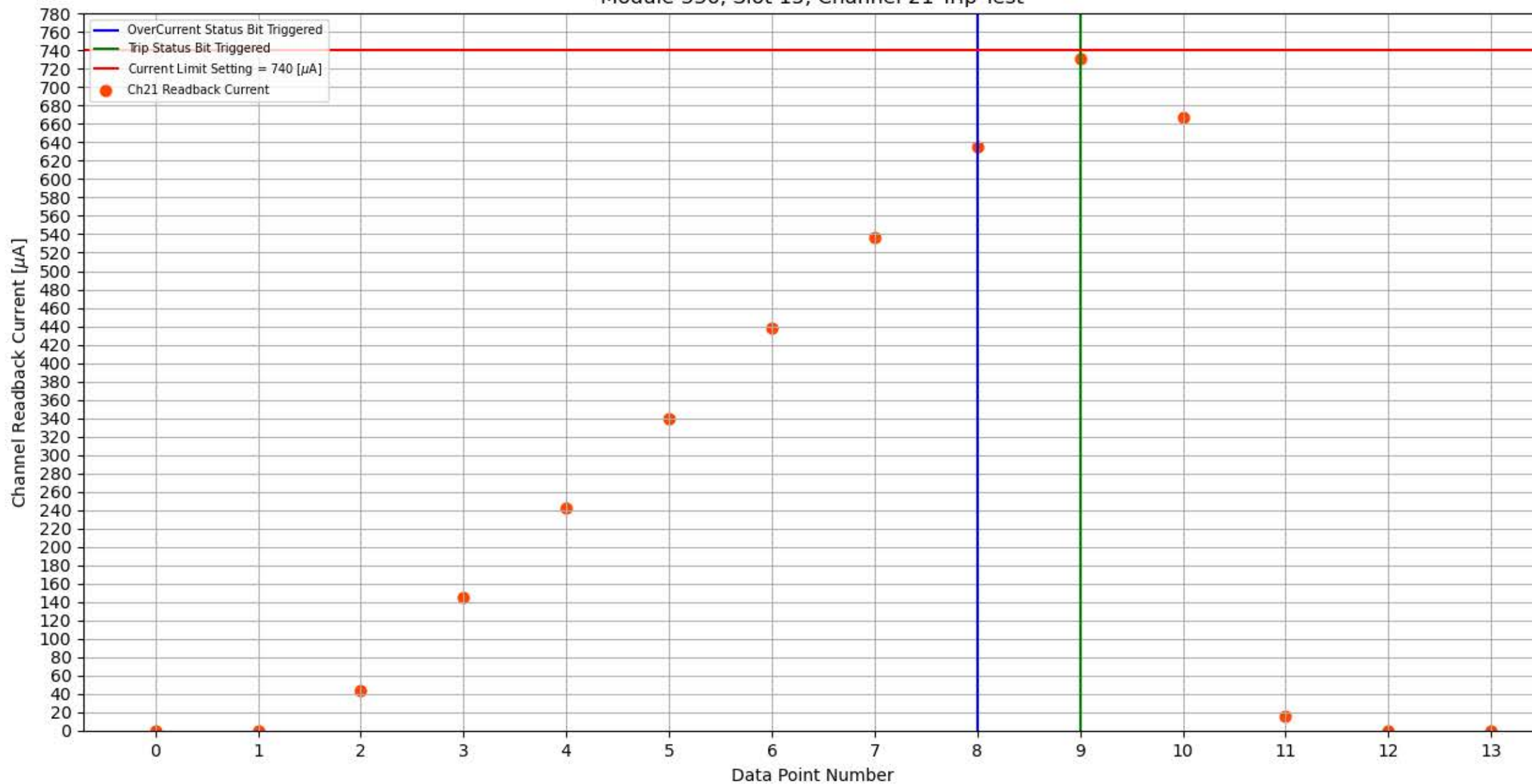
Module 336, Slot 15, Channel 21 Trip Test
