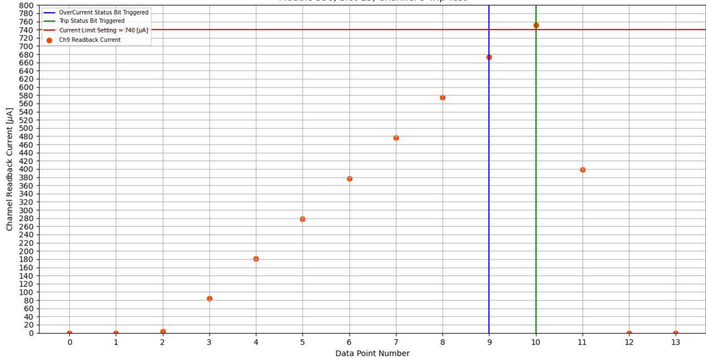
Module 336, Slot 15, Channel 9 Trip Test
