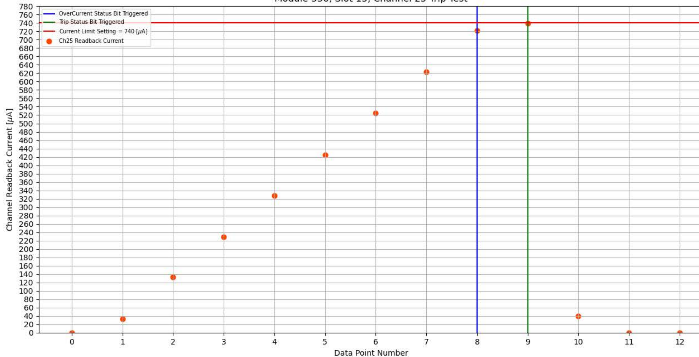
Module 336, Slot 15, Channel 25 Trip Test
