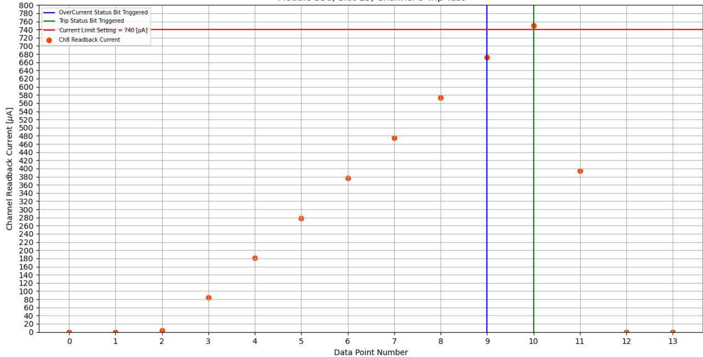
Module 336, Slot 15, Channel 8 Trip Test
