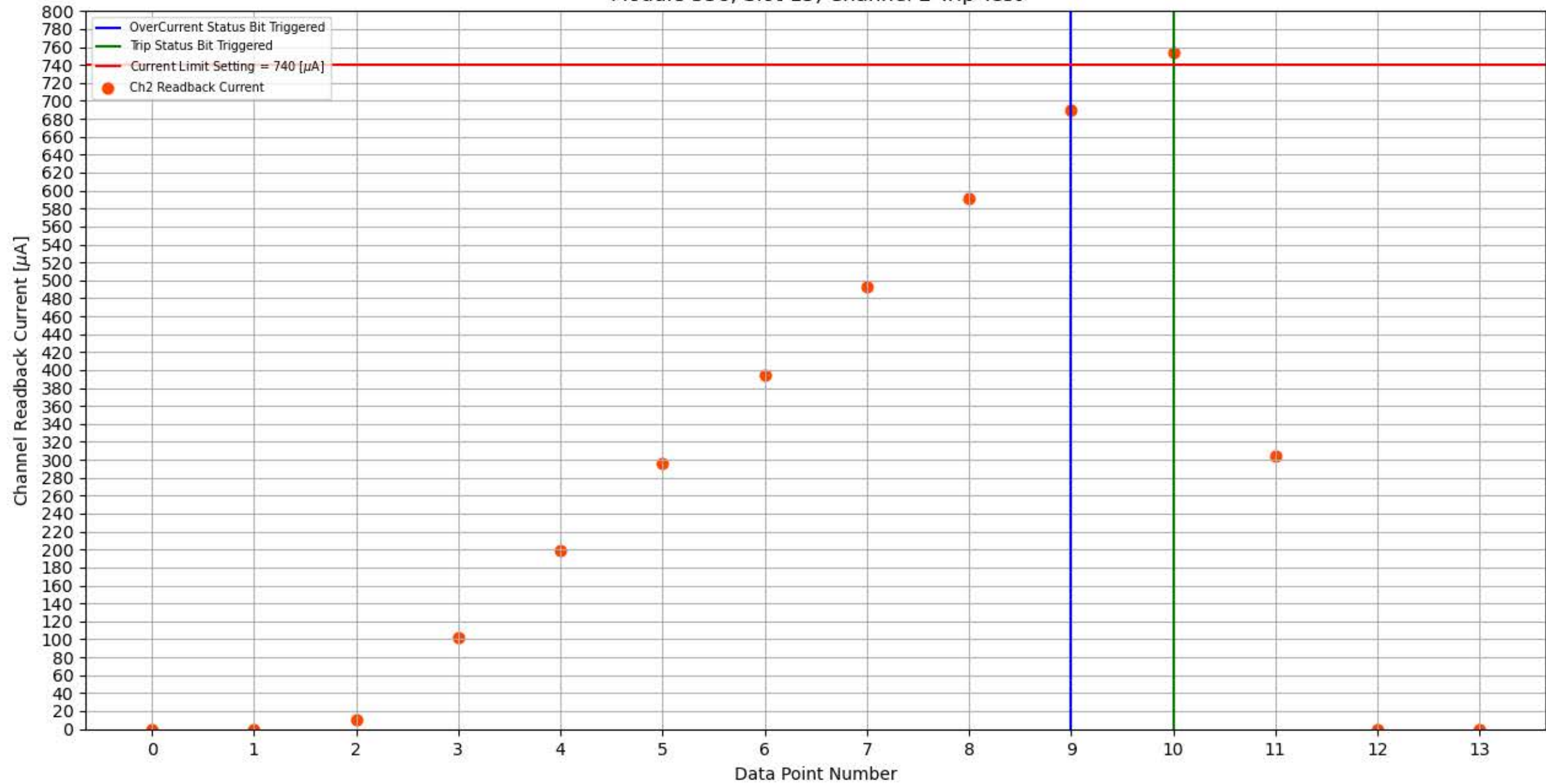
Module 336, Slot 15, Channel 2 Trip Test
