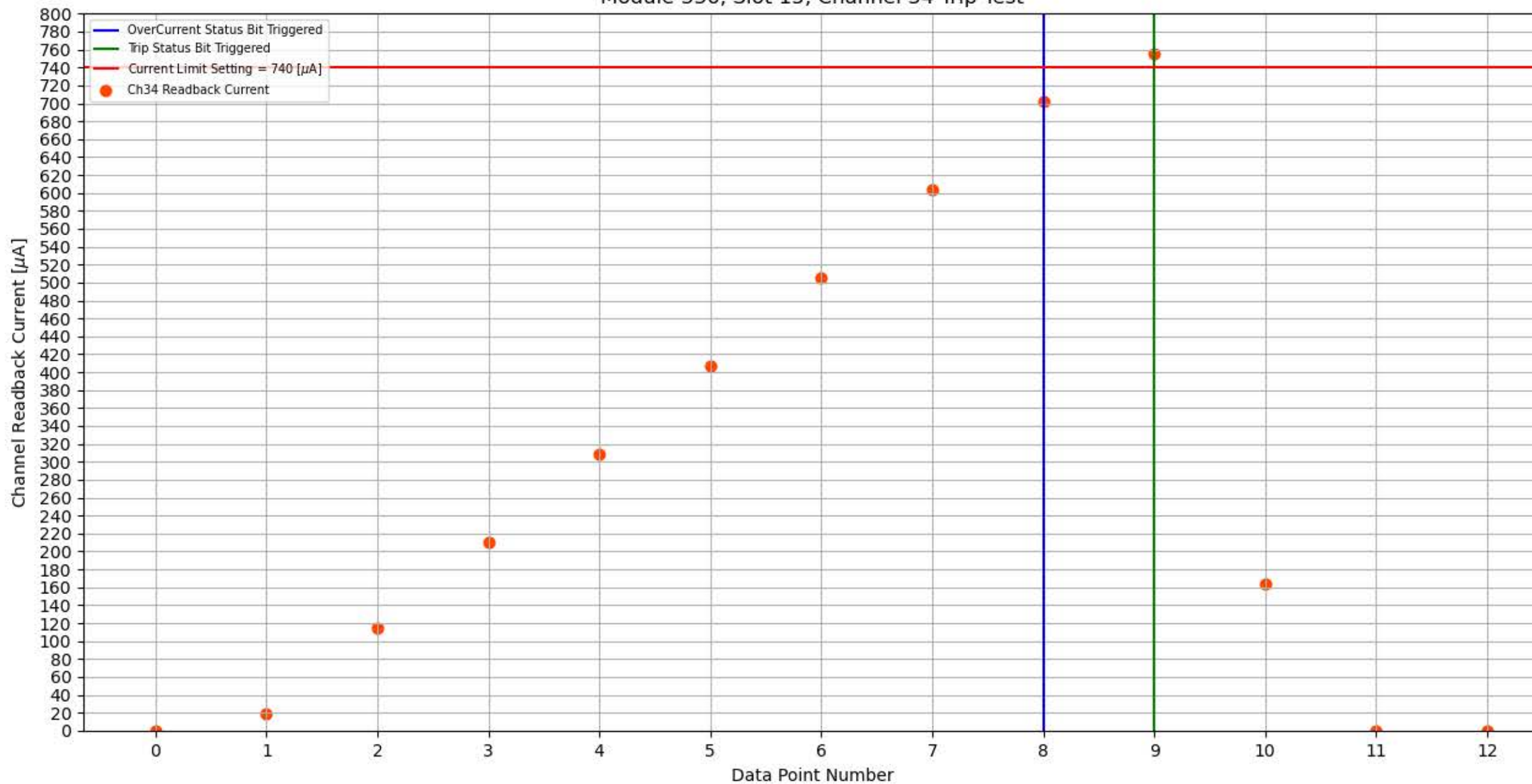
Module 336, Slot 15, Channel 34 Trip Test
