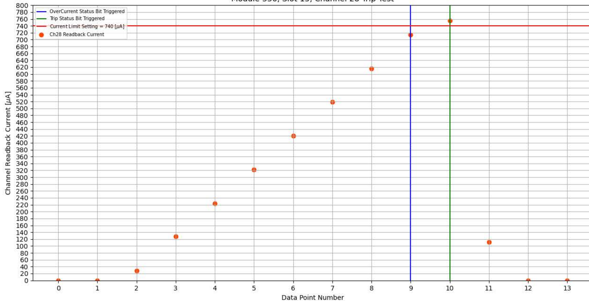
Module 336, Slot 15, Channel 28 Trip Test
