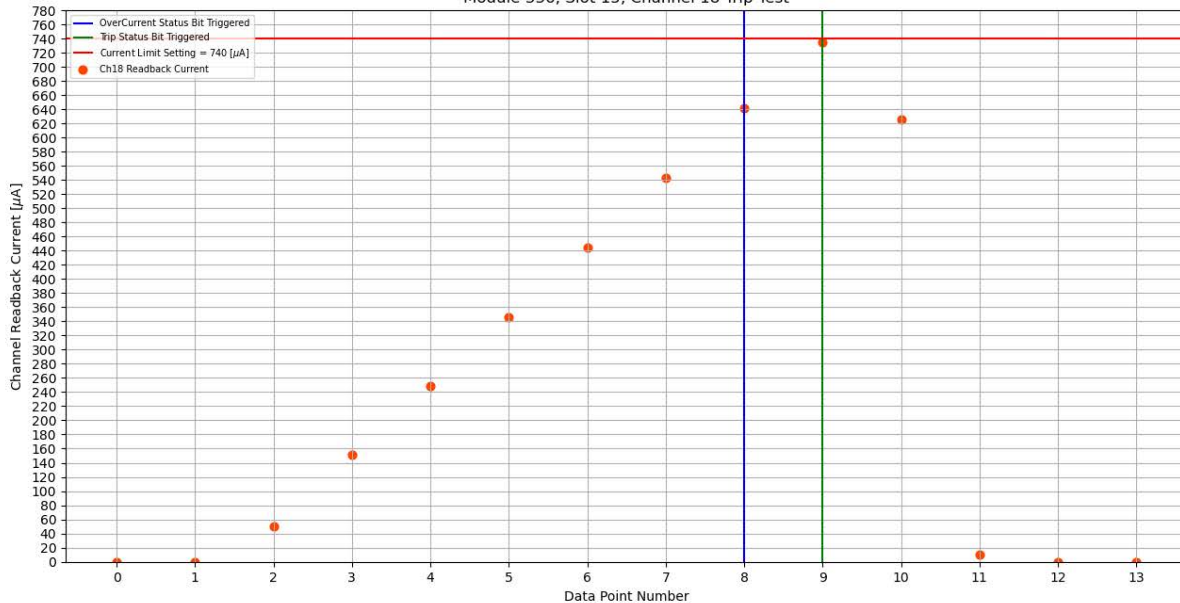
Module 336, Slot 15, Channel 18 Trip Test
